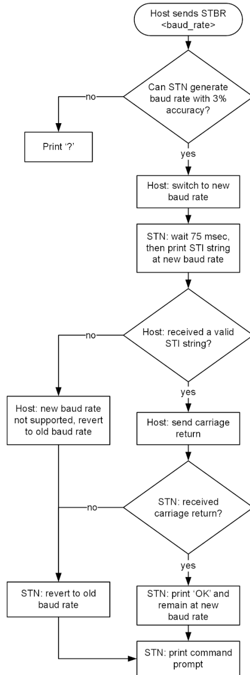
Figure 1 - STBR Algorithm
