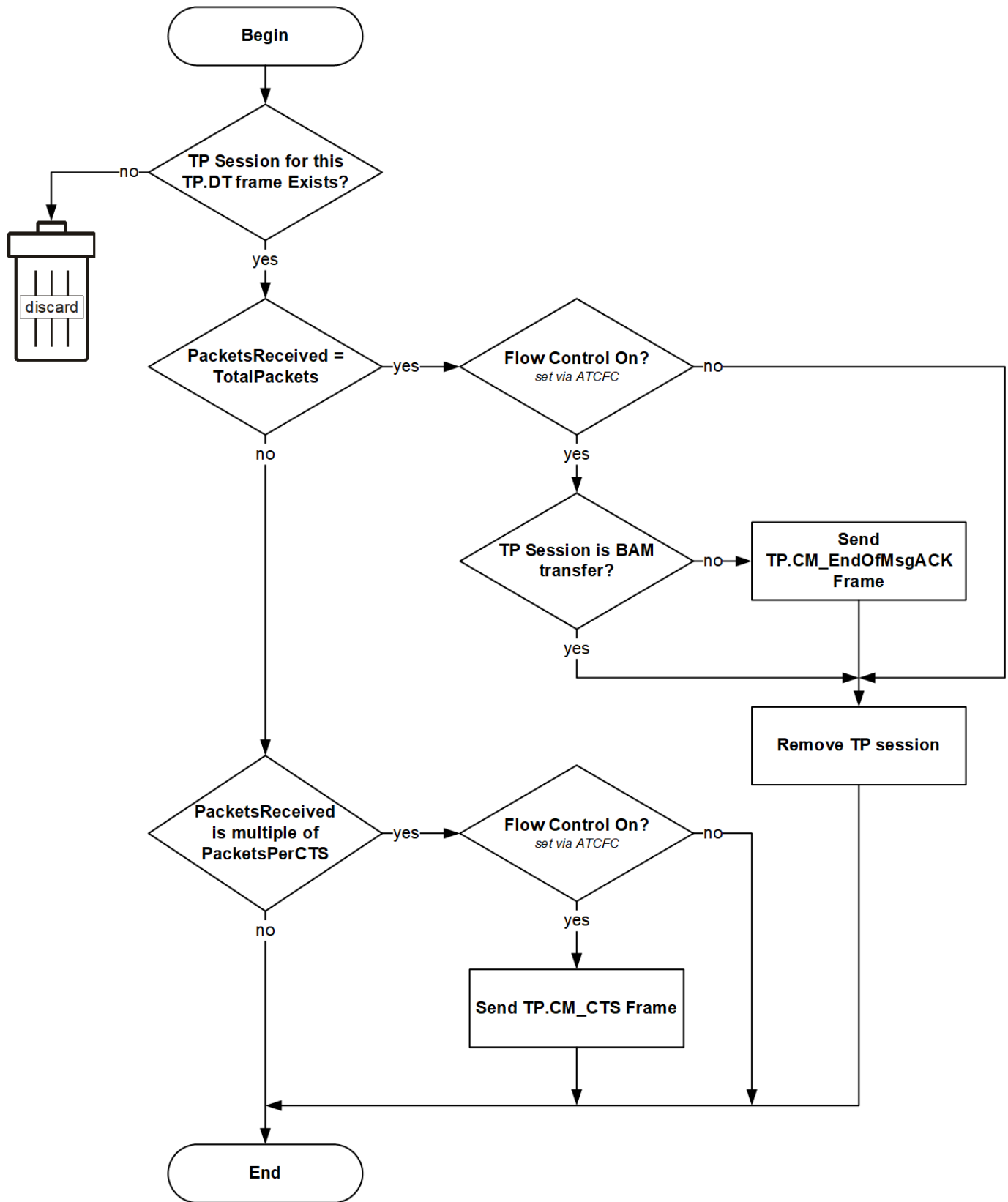
Figure 8 – Process TP.DT Frame
